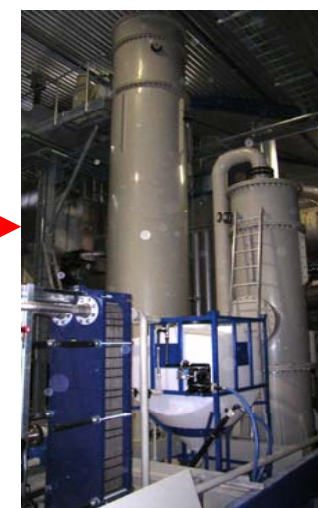
CO 2 RECOVERY INSTALLATIE
